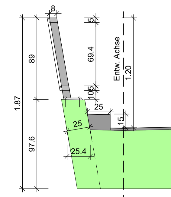
Detail A M 1:25
